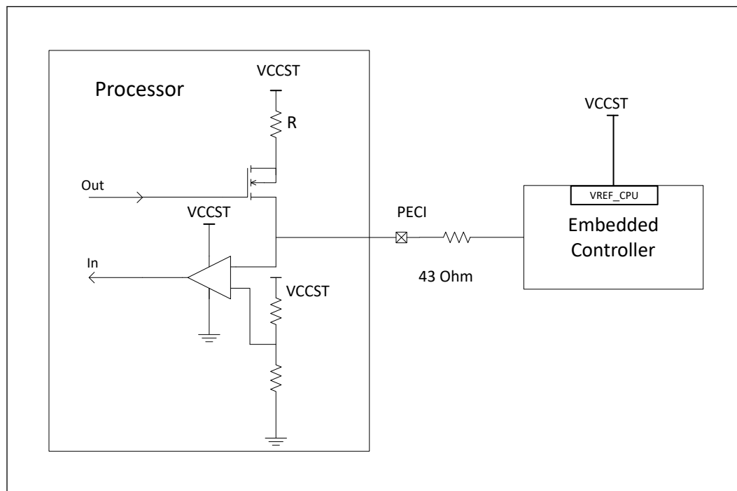
Figure 7. Example for PECE EC Connection
