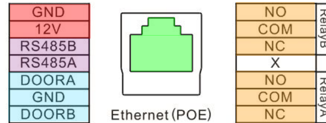
Figure 1.2.1 Connector Introduction
