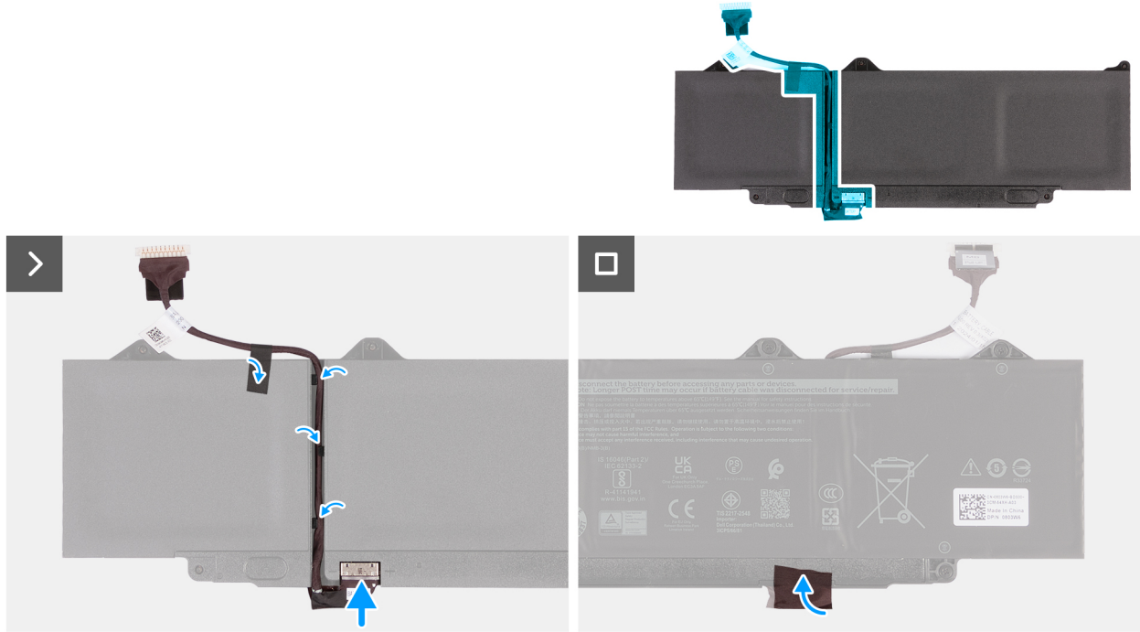
Figure 31. Installing the battery cable
