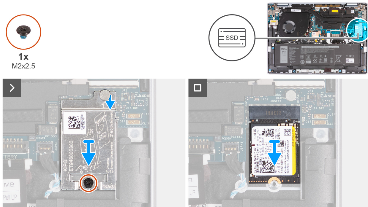
Figure 16. Removing the SSD
