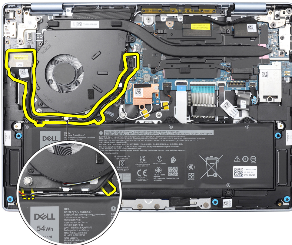
Figure 38. Location of the I/O-board cable
