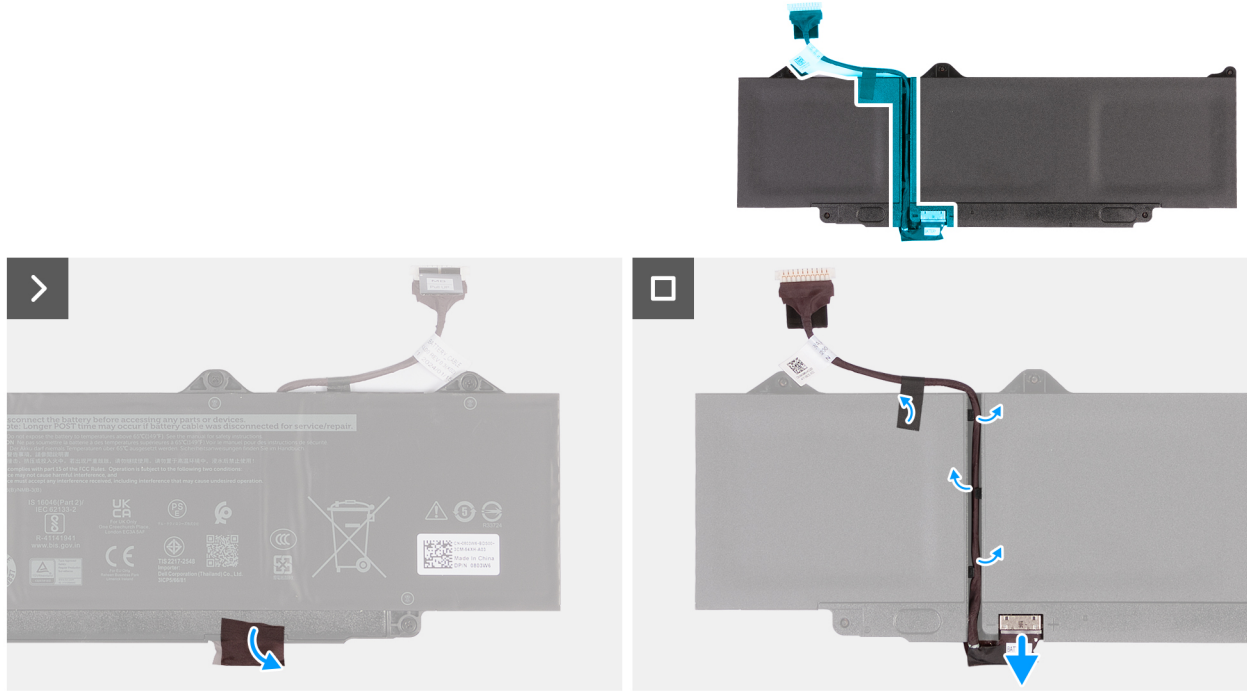
Figure 29. Removing the battery cable
