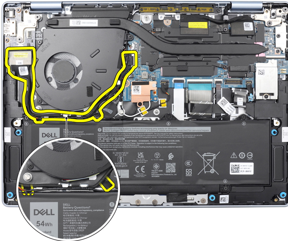
Figure 36. Location of the I/O-board cable
