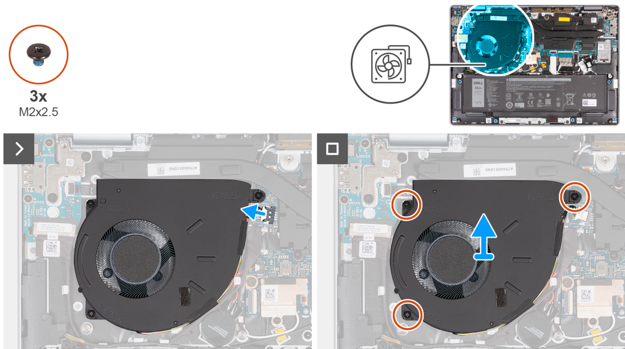
Figure 25. Removing the fan
