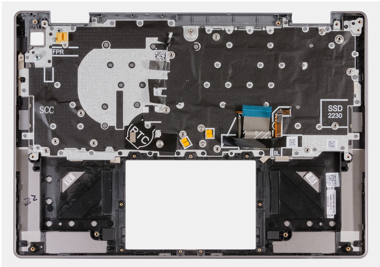
Figure 66. Palm-rest and keyboard assembly
