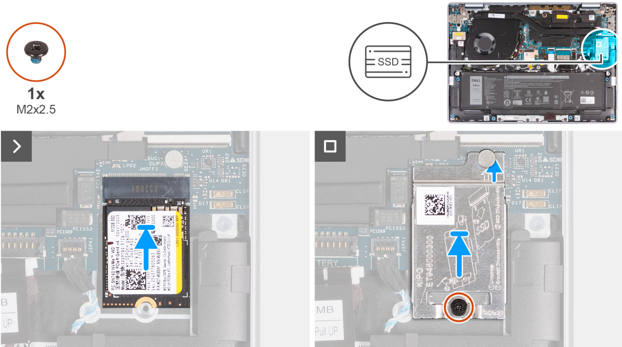
Figure 18. Installing the SSD
