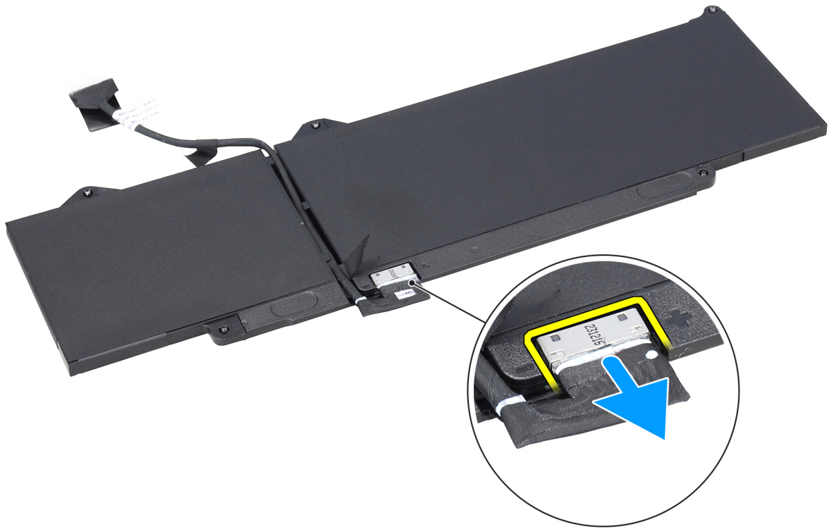
Figure 30. Disconnecting the battery cable
