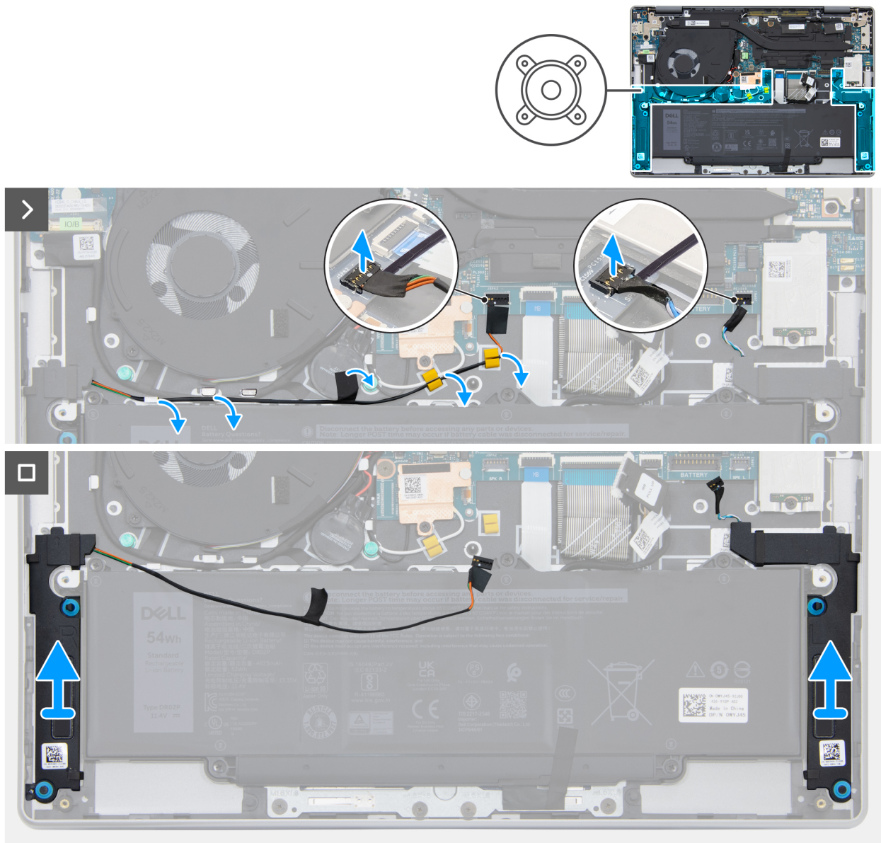
Figure 21. Removing the speakers
