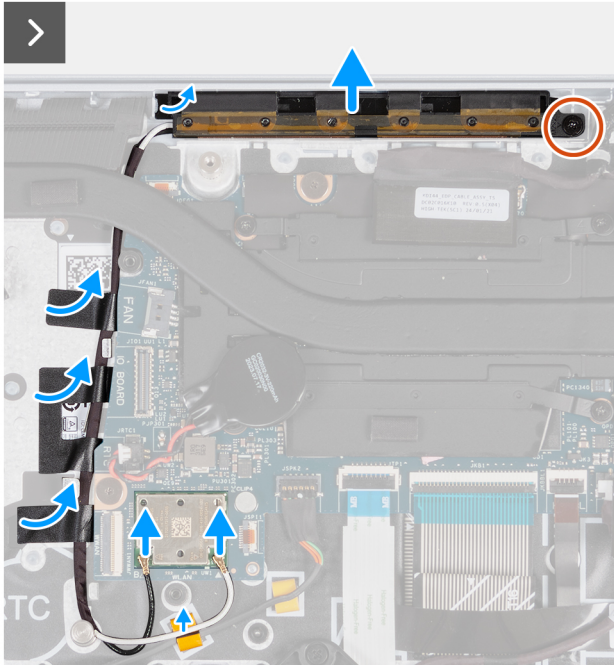
Figure 40. Removing the WLAN-antenna module
