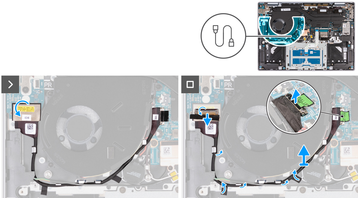
Figure 37. Removing the I/O-board cable
