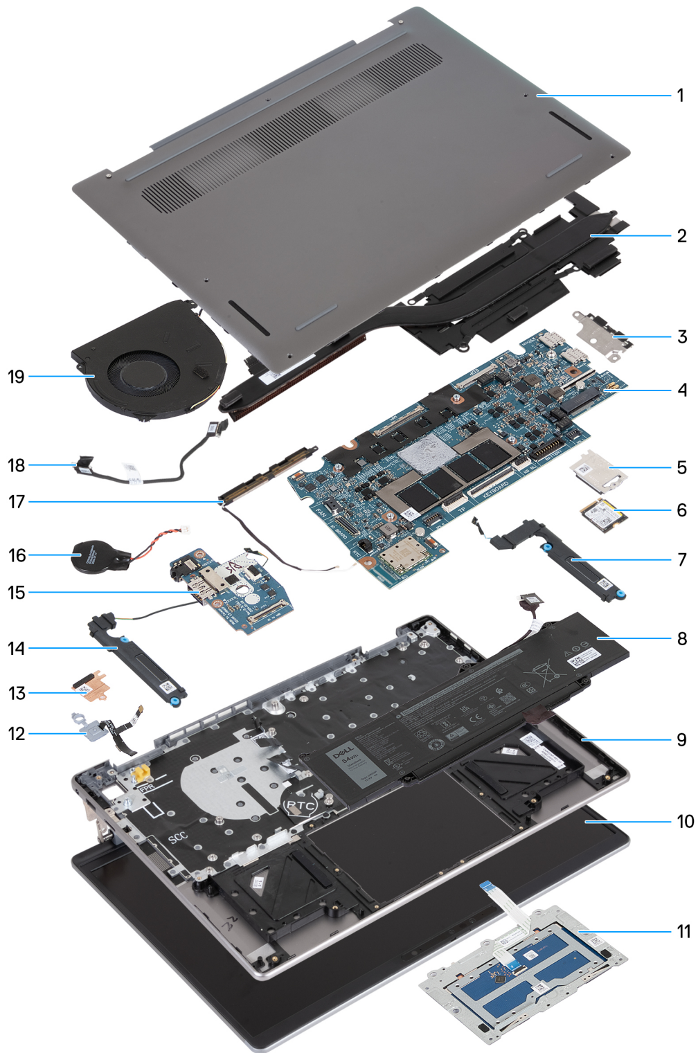
Figure 9. Major components of Latitude 5455
