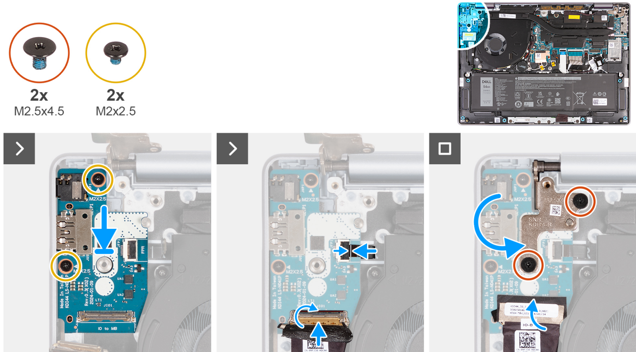
Figure 51. Installing the I/O board
