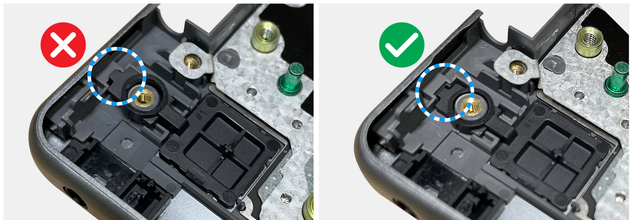
Figure 58. Installing the power button
