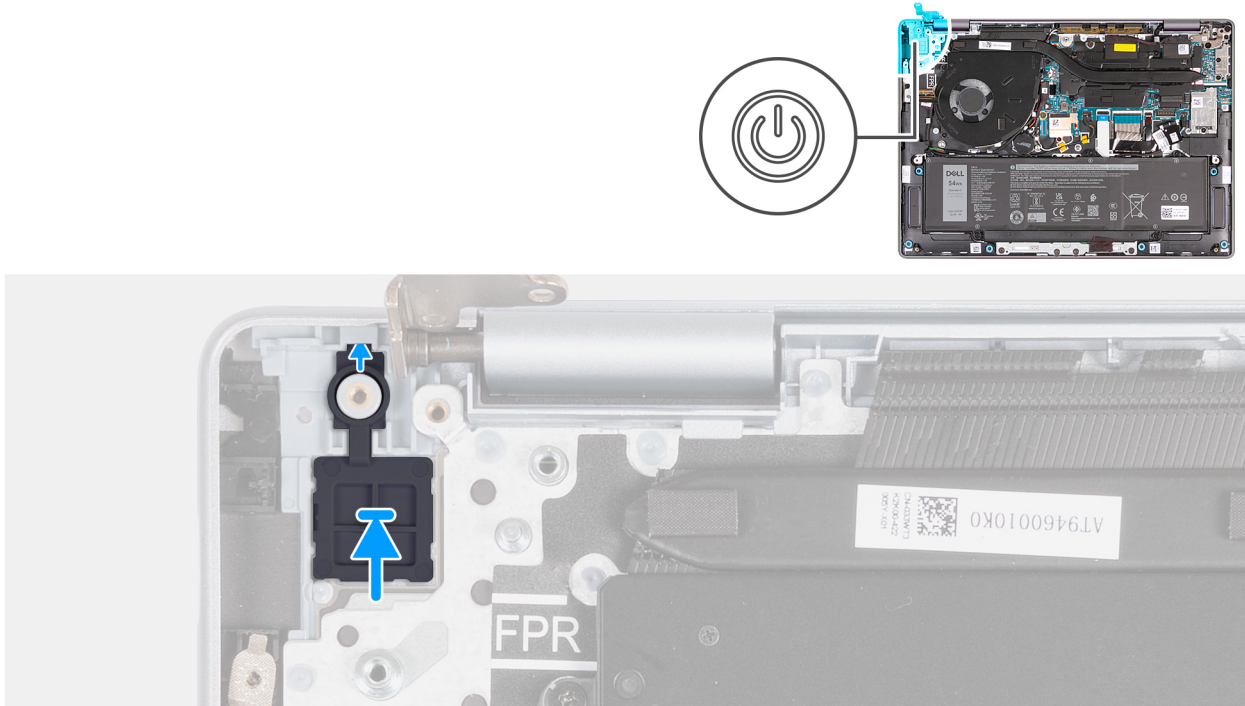
Figure 56. Installing the power button
