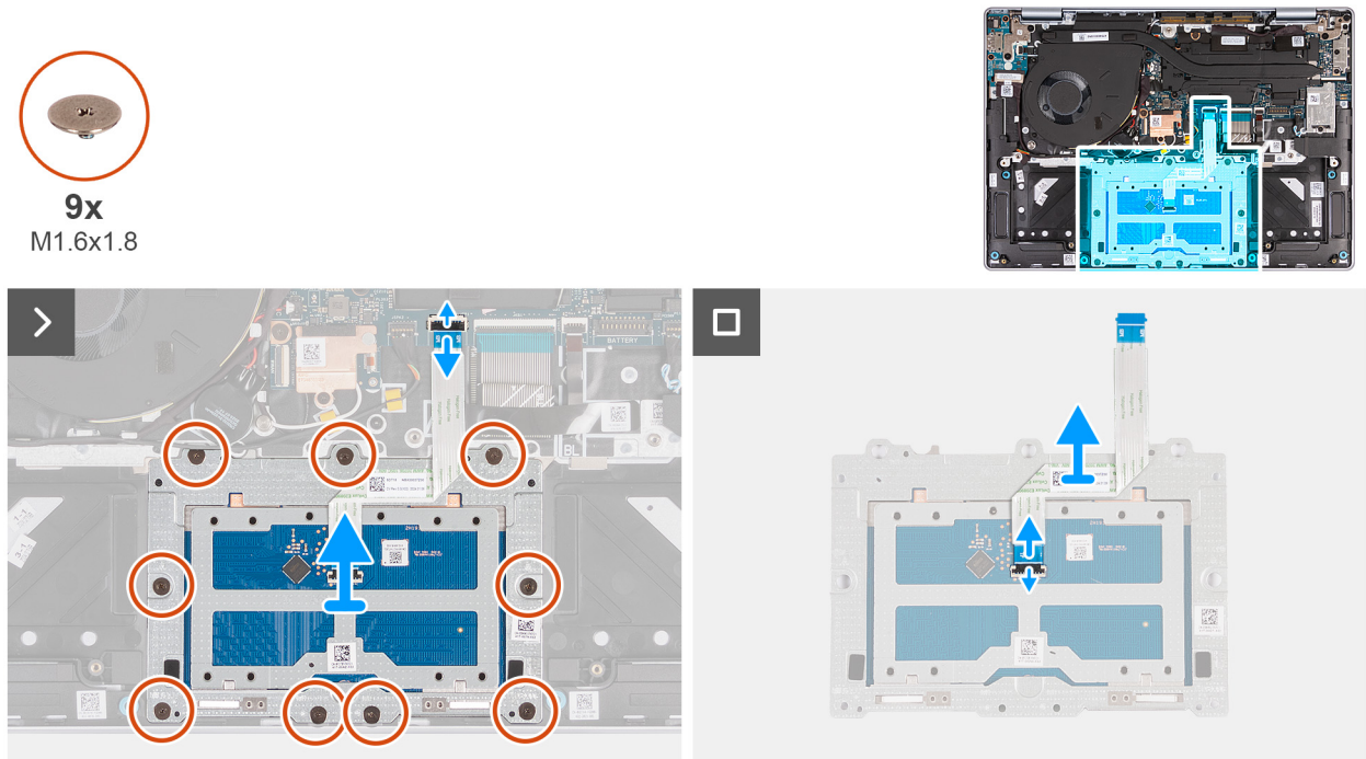
Figure 52. Removing the touchpad assembly
