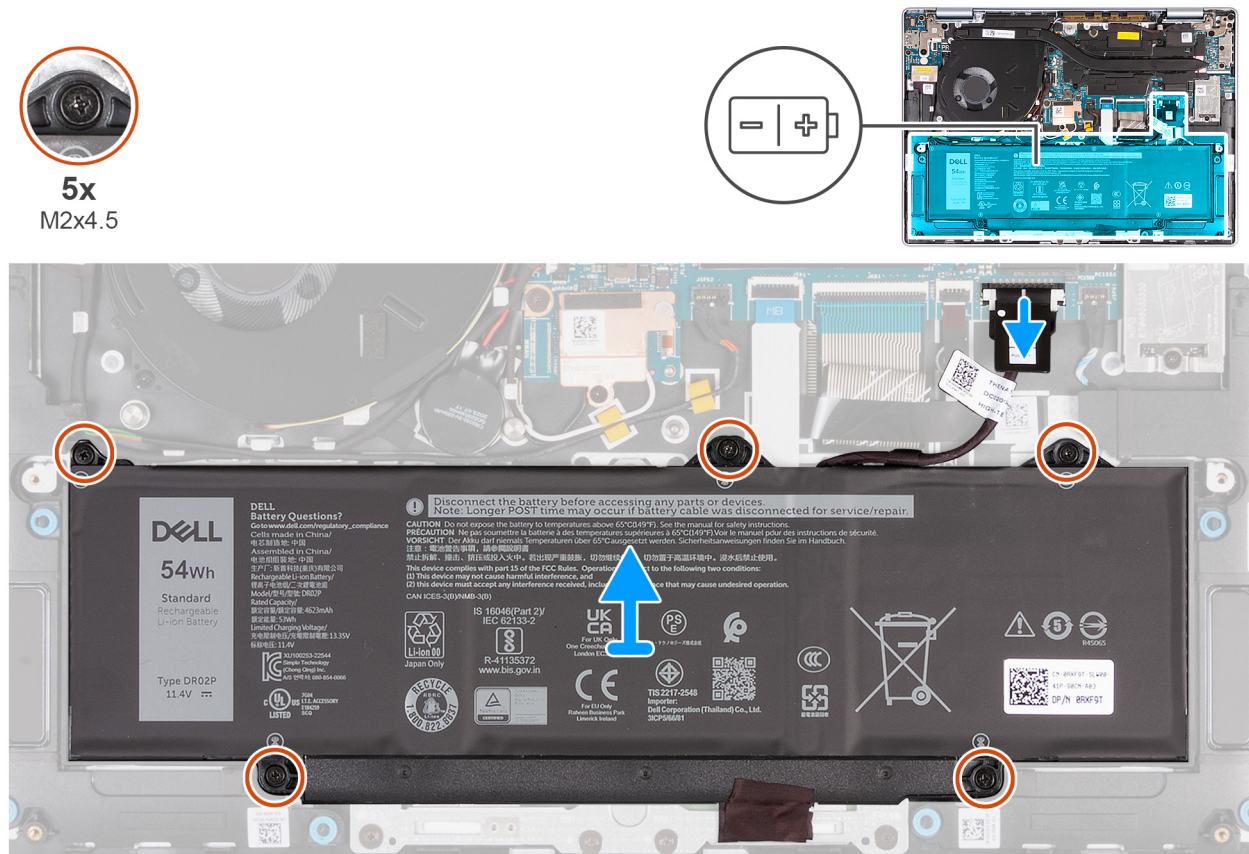
Figure 27. Removing the battery
