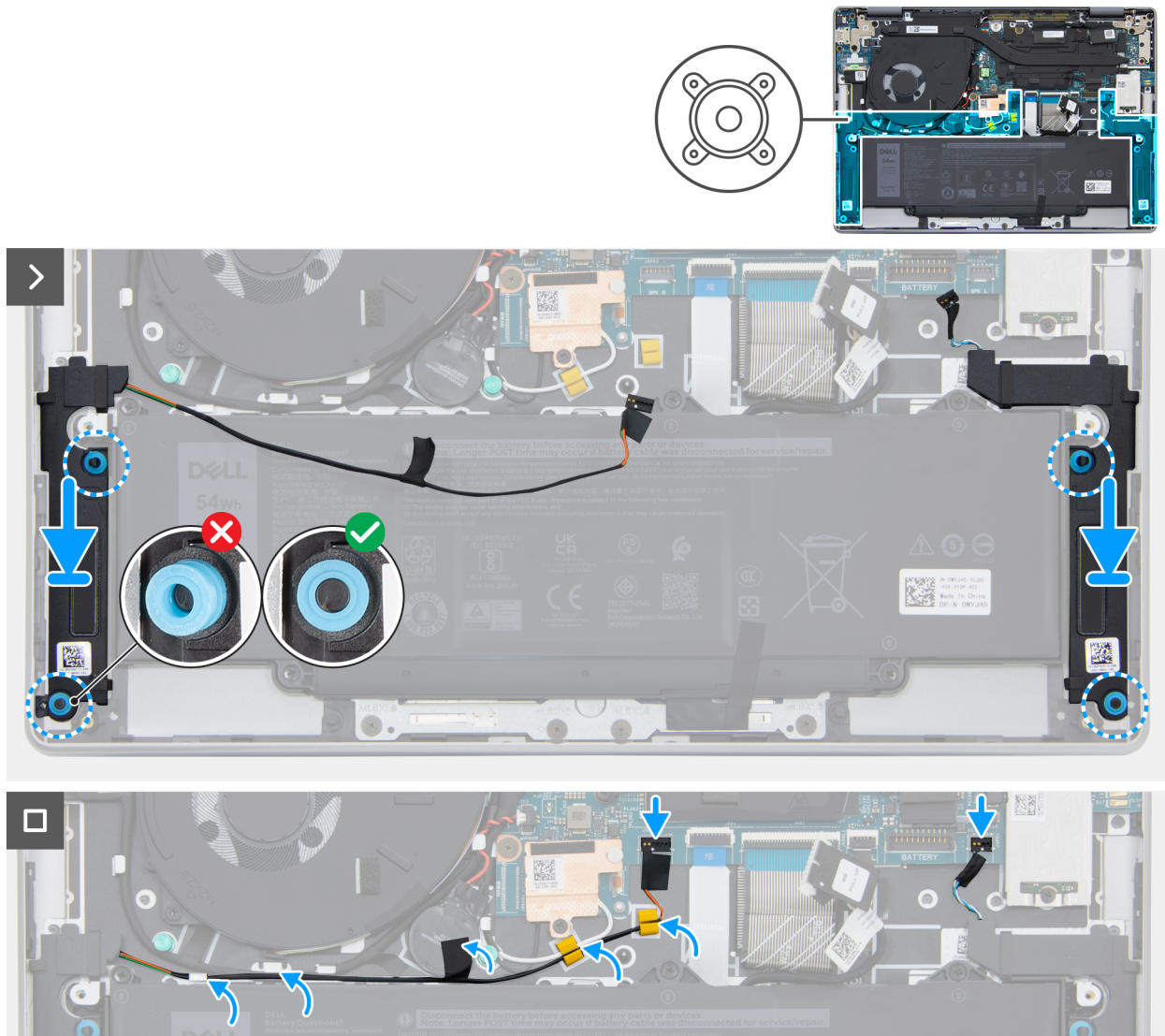
Figure 23. Installing the speakers
