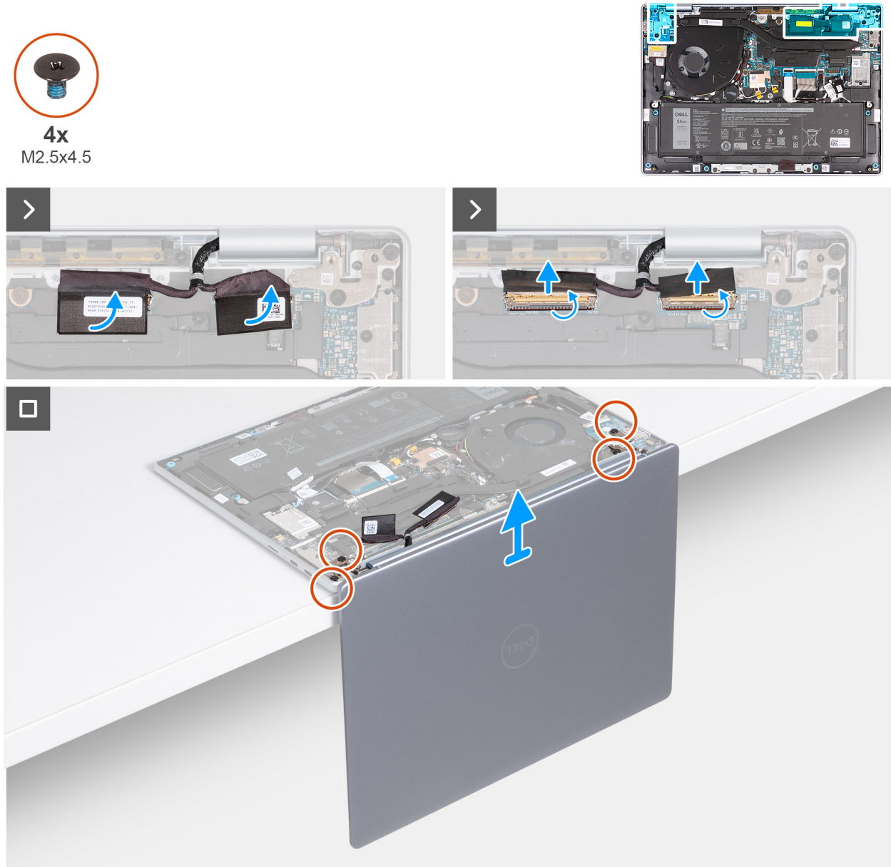
Figure 47. Removing the display assembly
