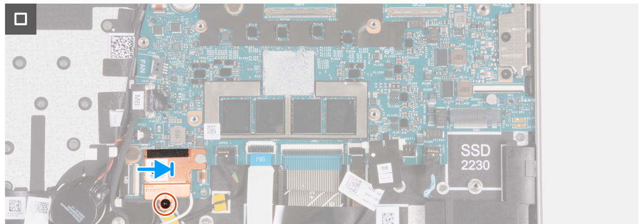
Figure 65. Installing the system board
