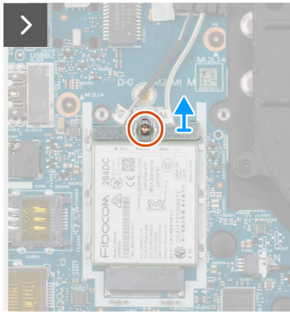
Figure 30. Removing the 4G WWAN card
