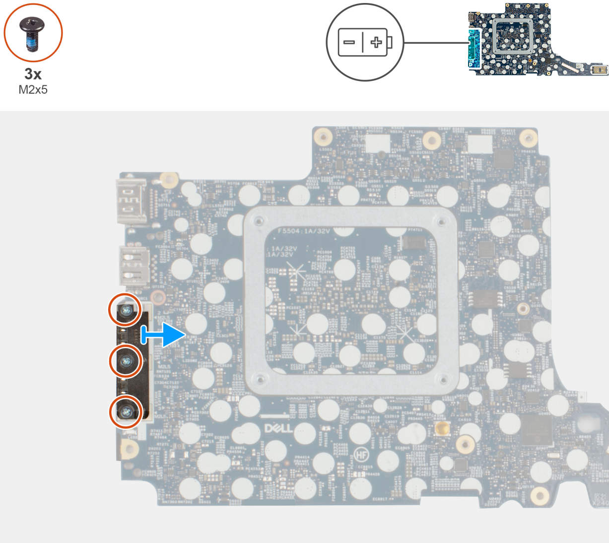
Figure 50. Removing the USB Type-C connector module
