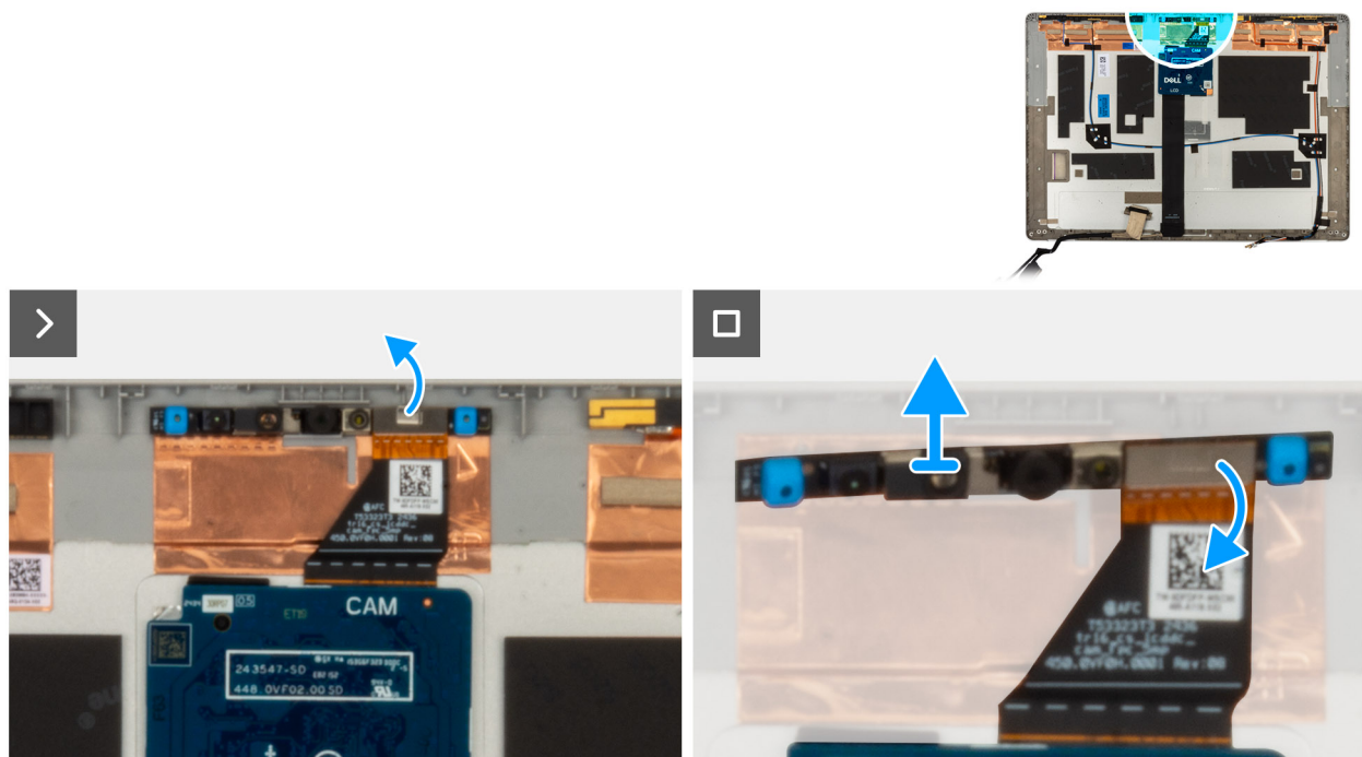
Figure 74. Removing the camera module
