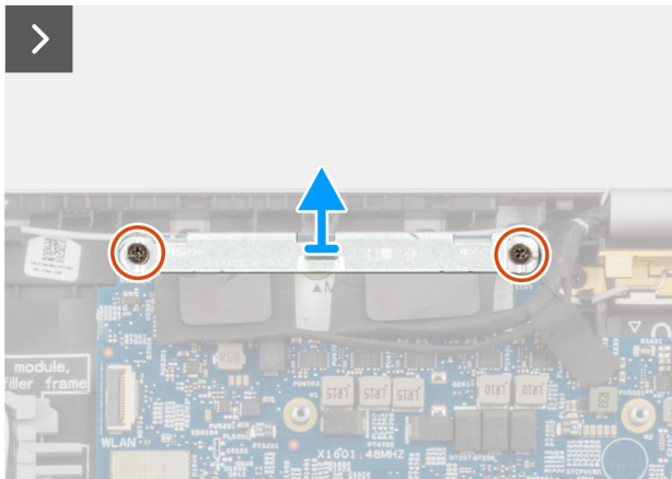
Figure 54. Removing the display assembly
