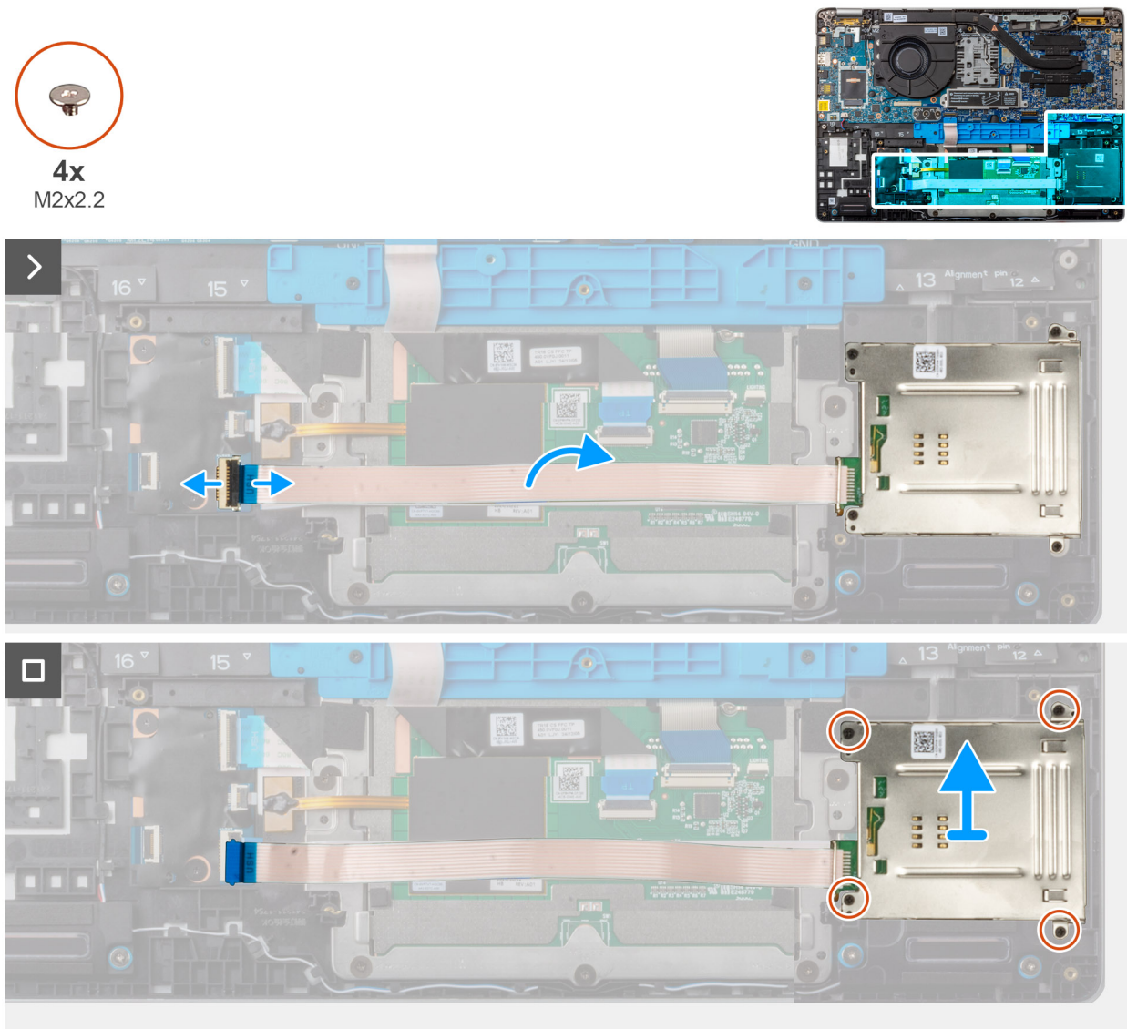
Figure 38. Removing the Smart card reader
