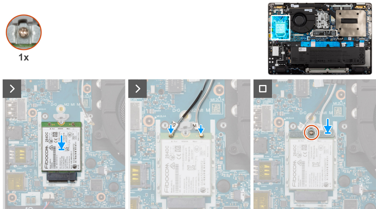
Figure 31. Installing the 4G WWAN card
