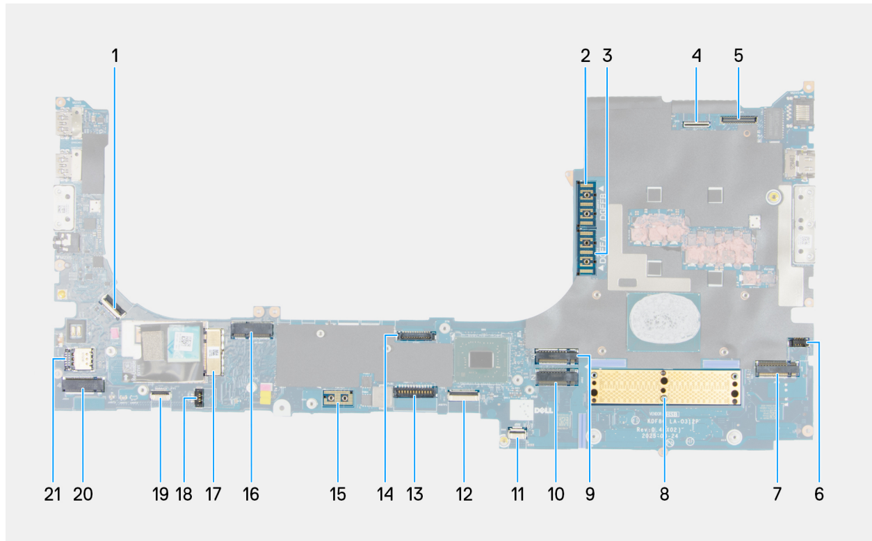
Figure 110. System-board components
