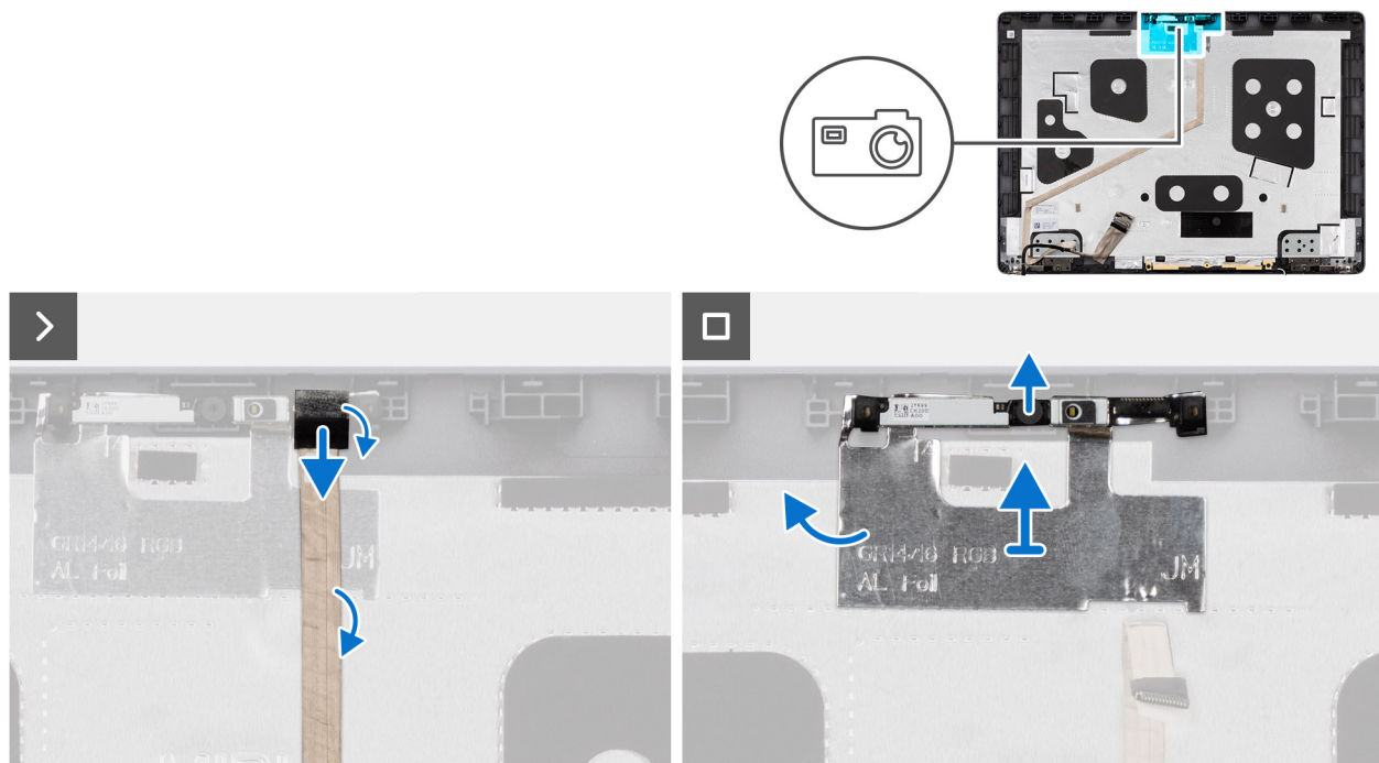
Figure 69. Removing the camera
