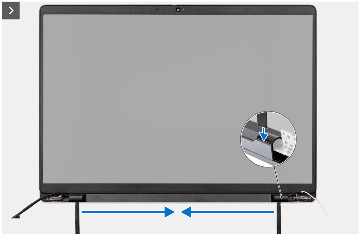
Figure 53. Removing the display bezel
