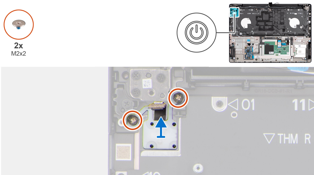
Figure 81. Removing the power button
