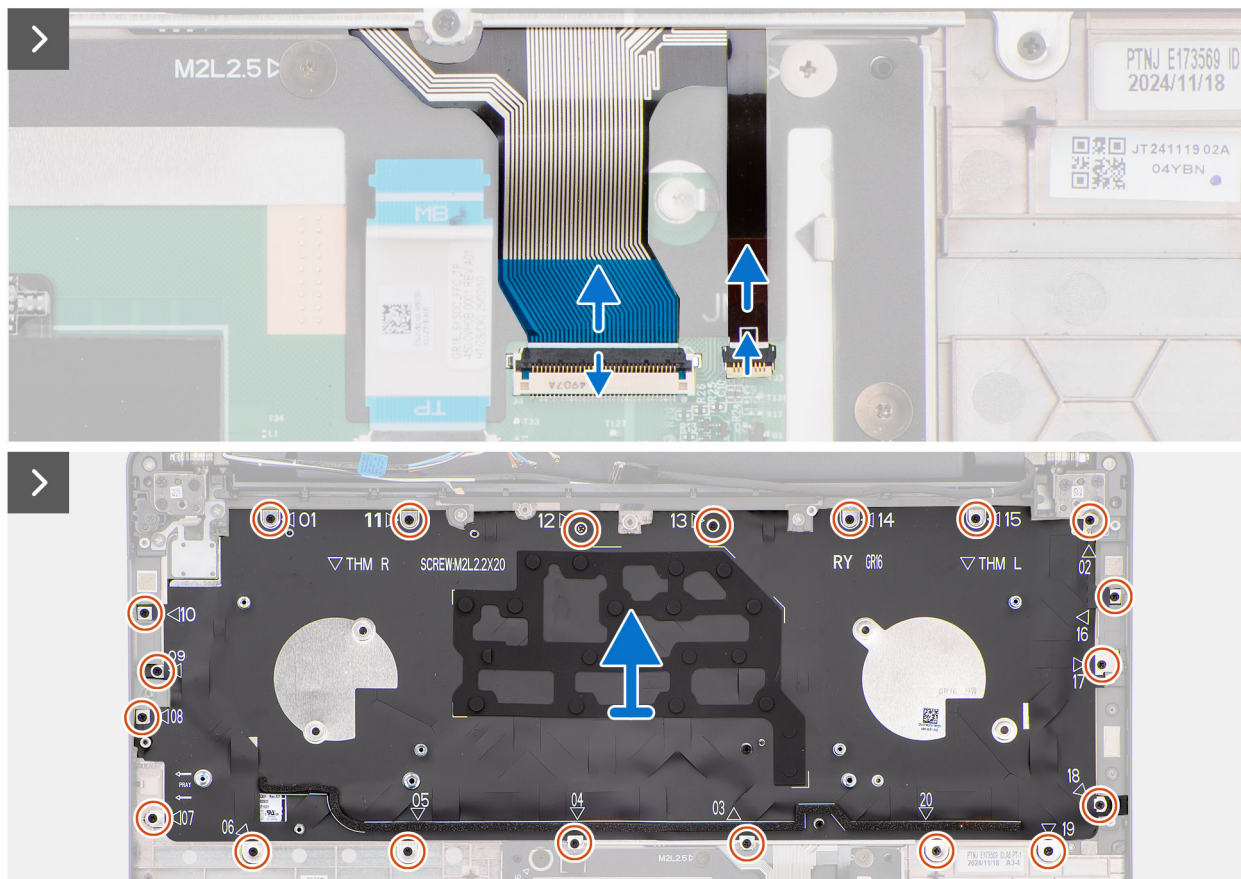
Figure 83. Removing the keyboard
