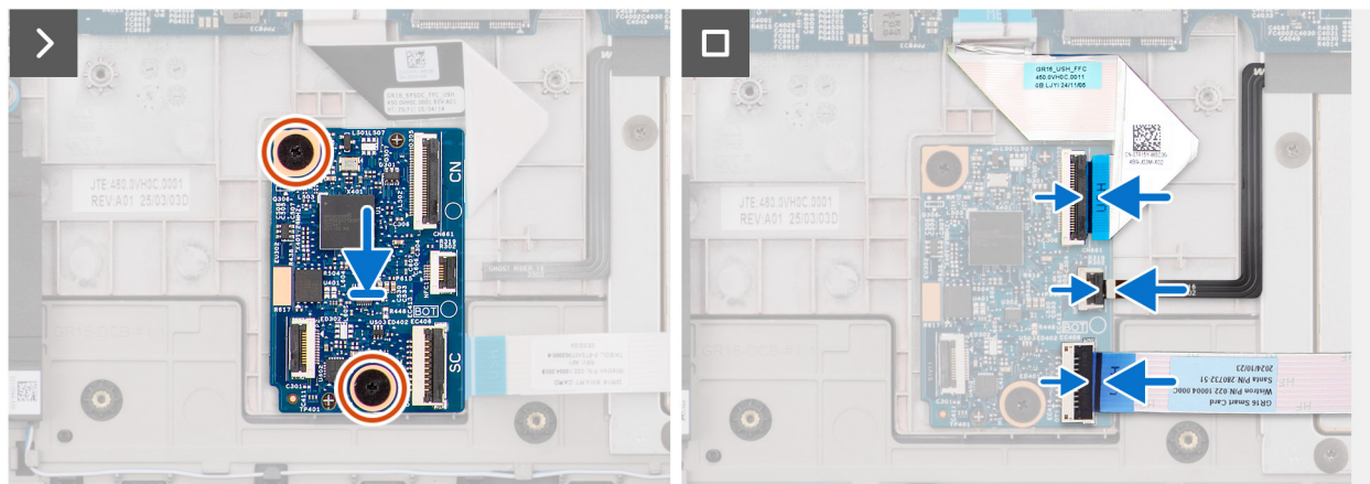
Figure 41. Installing the USH board
