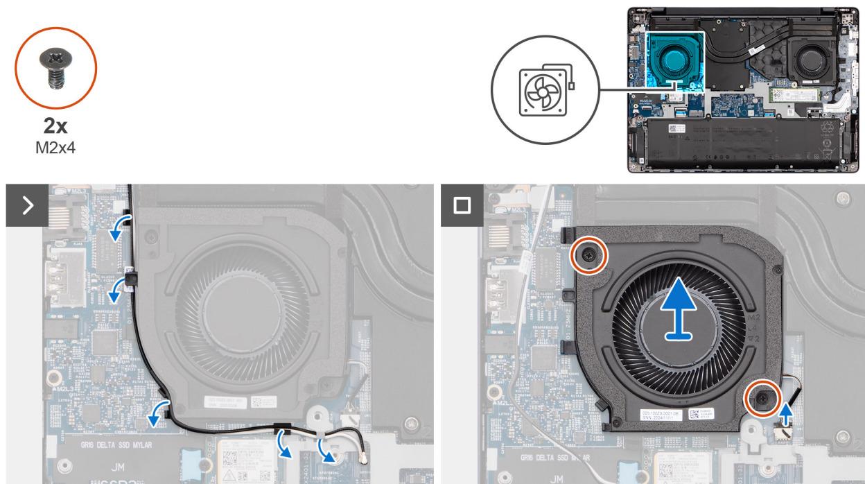
Figure 30. Removing the right/processor fan
