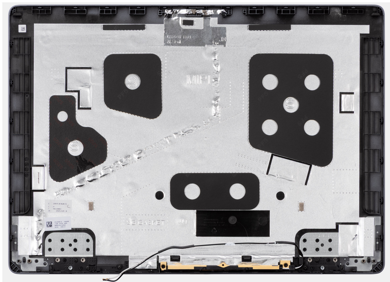
Figure 71. Display back-cover and antenna assembly
