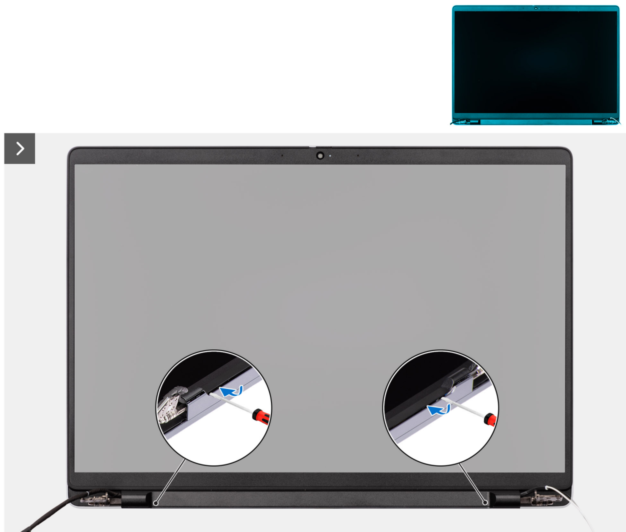
Figure 50. Removing the display bezel
