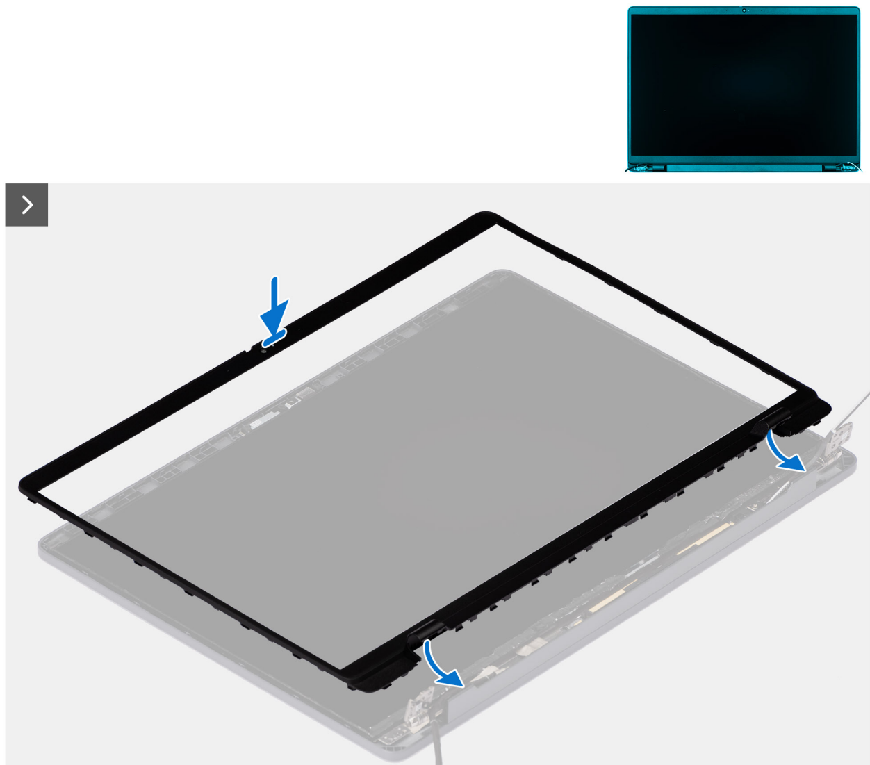
Figure 56. Installing the display bezel
