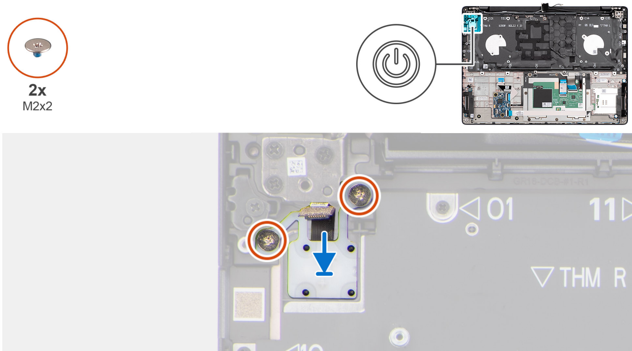
Figure 82. Installing the power button
