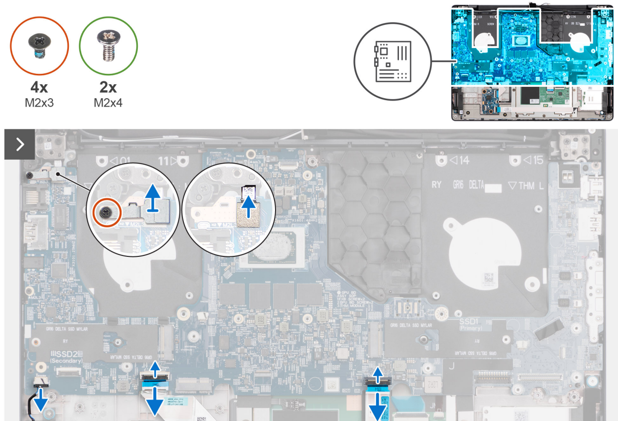
Figure 74. Removing the system board
