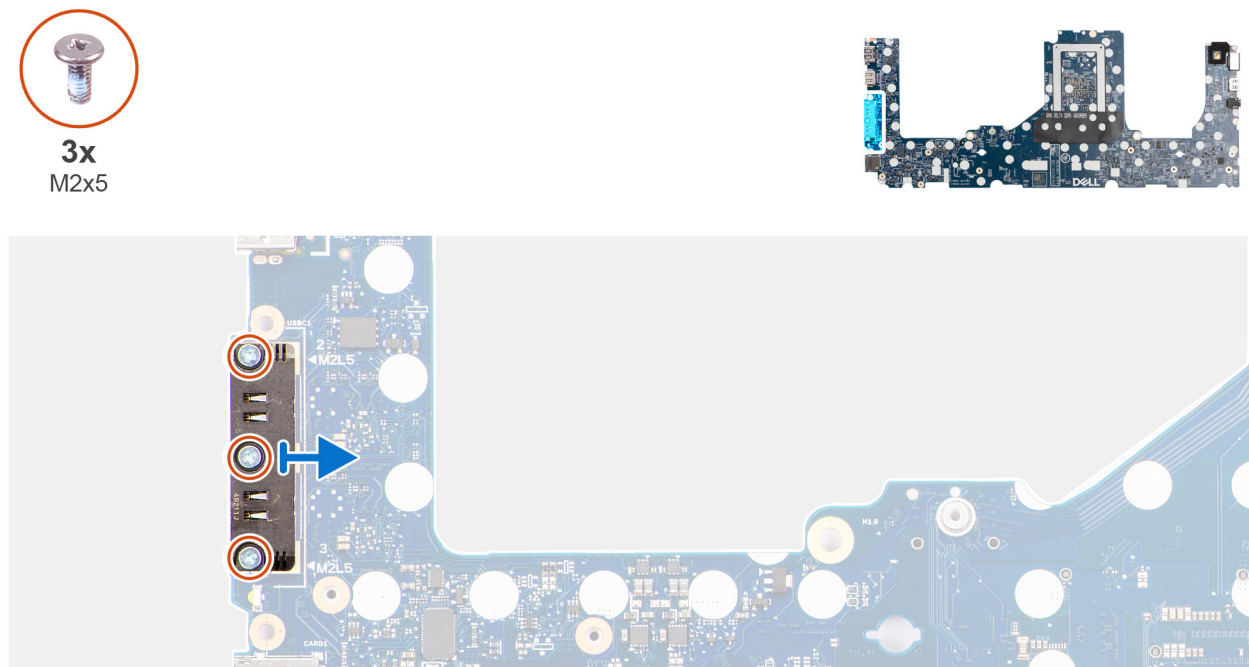
Figure 79. Removing the USB Type-C module
