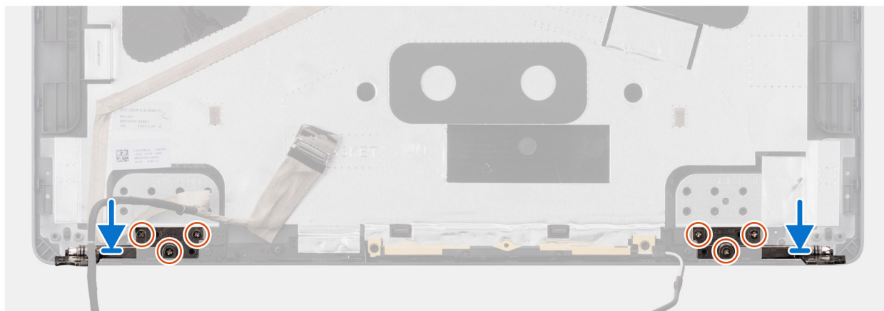
Figure 66. Installing the display hinges
