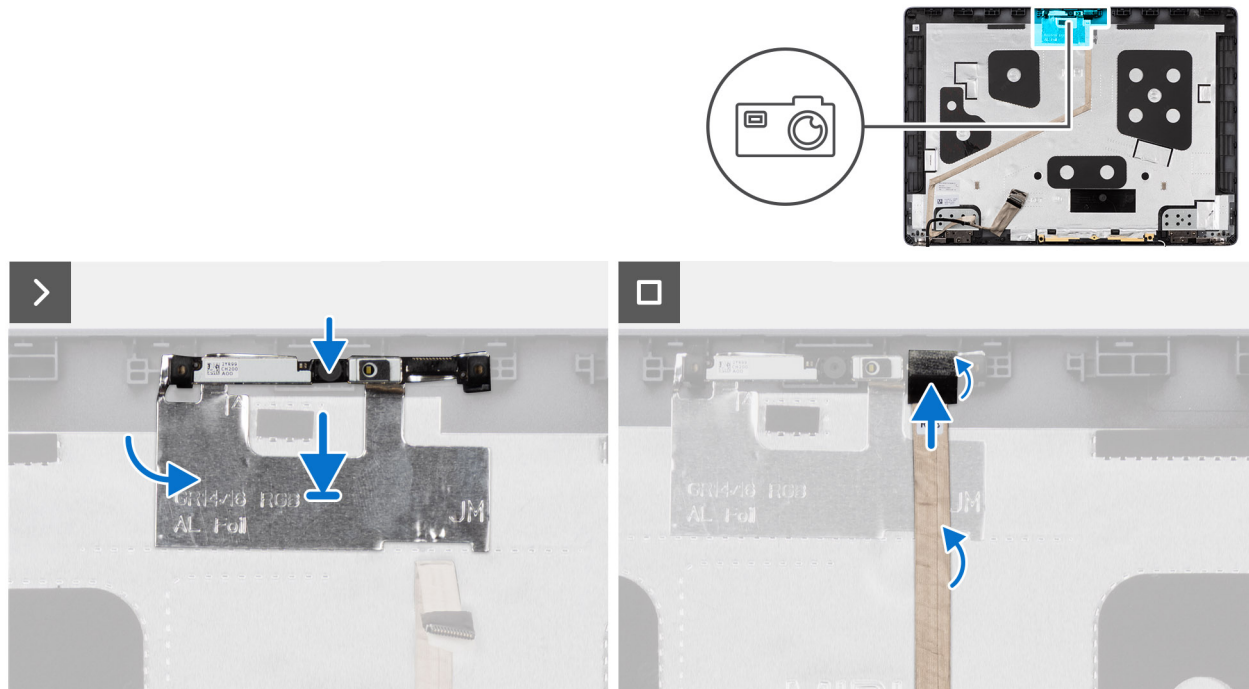
Figure 70. Installing the camera
