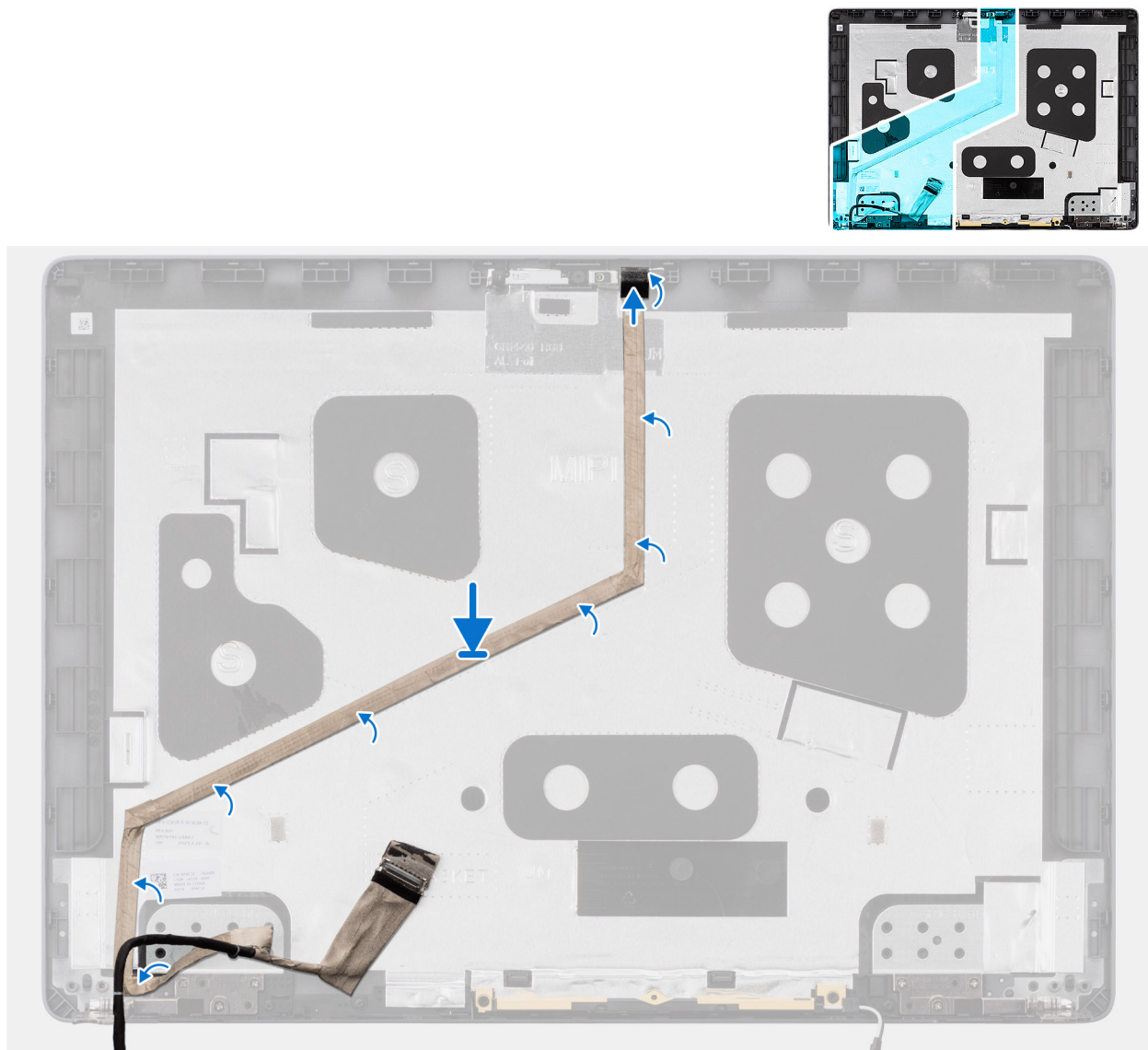
Figure 68. Installing the display cable
