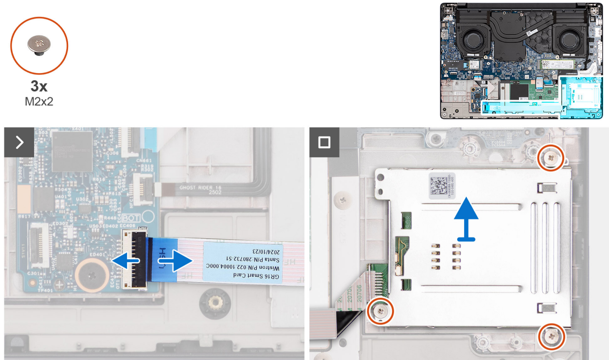
Figure 42. Removing the smart-card reader
