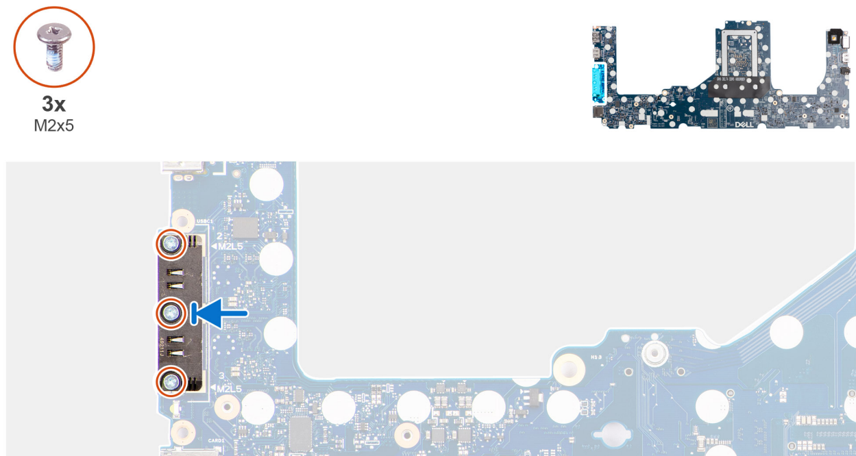
Figure 80. Installing the USB Type-C module
