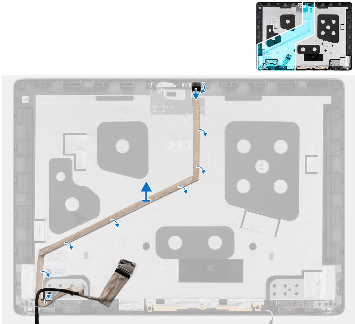
Figure 67. Removing the display cable
